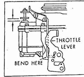
PUMP ADJ. Fig.4
