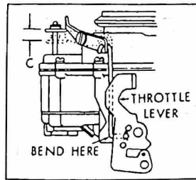
PUMP ADJ. Fig.3
