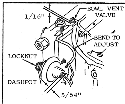
BOWL VENT AND DASHPOT Fig. 3 ADJUSTMENT
