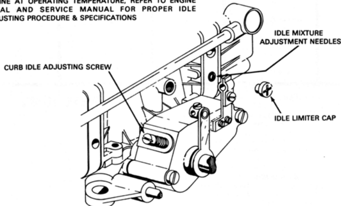
SLOW IDLE ADJUSTMENT
