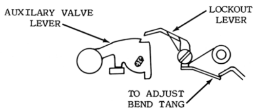
AUXILIARY THROTTLE VALVE LOCKOUT ADJUSTMENT
