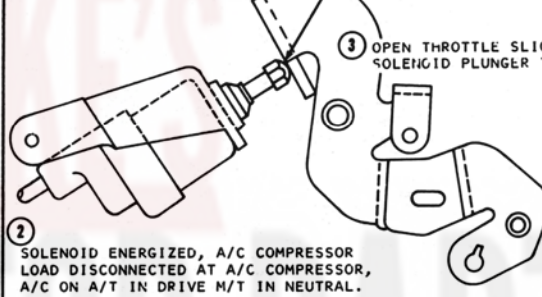
A/C IDLE SPEED UP SOLENOID ADJUSTMENT
